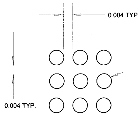
HOLE PATTERN
